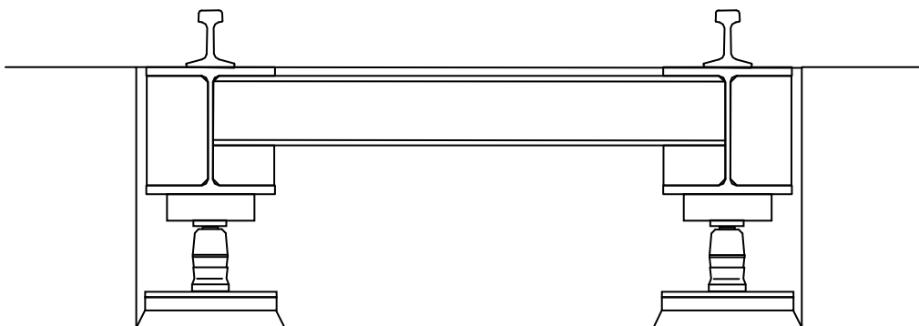
7260 Cross Section
